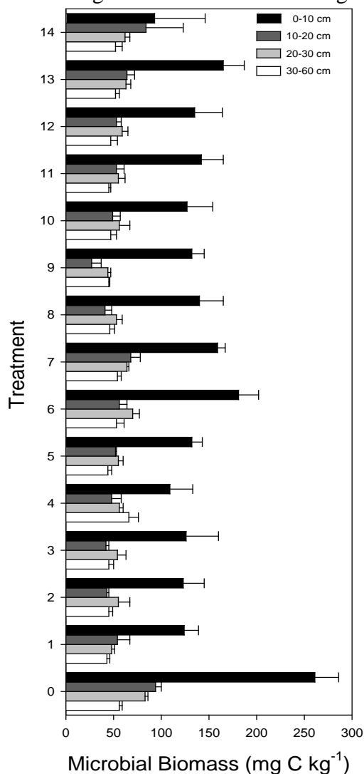
Figure 1. Microbial biomass C as a function of management treatment and depth. Bars are means with standard errors.
