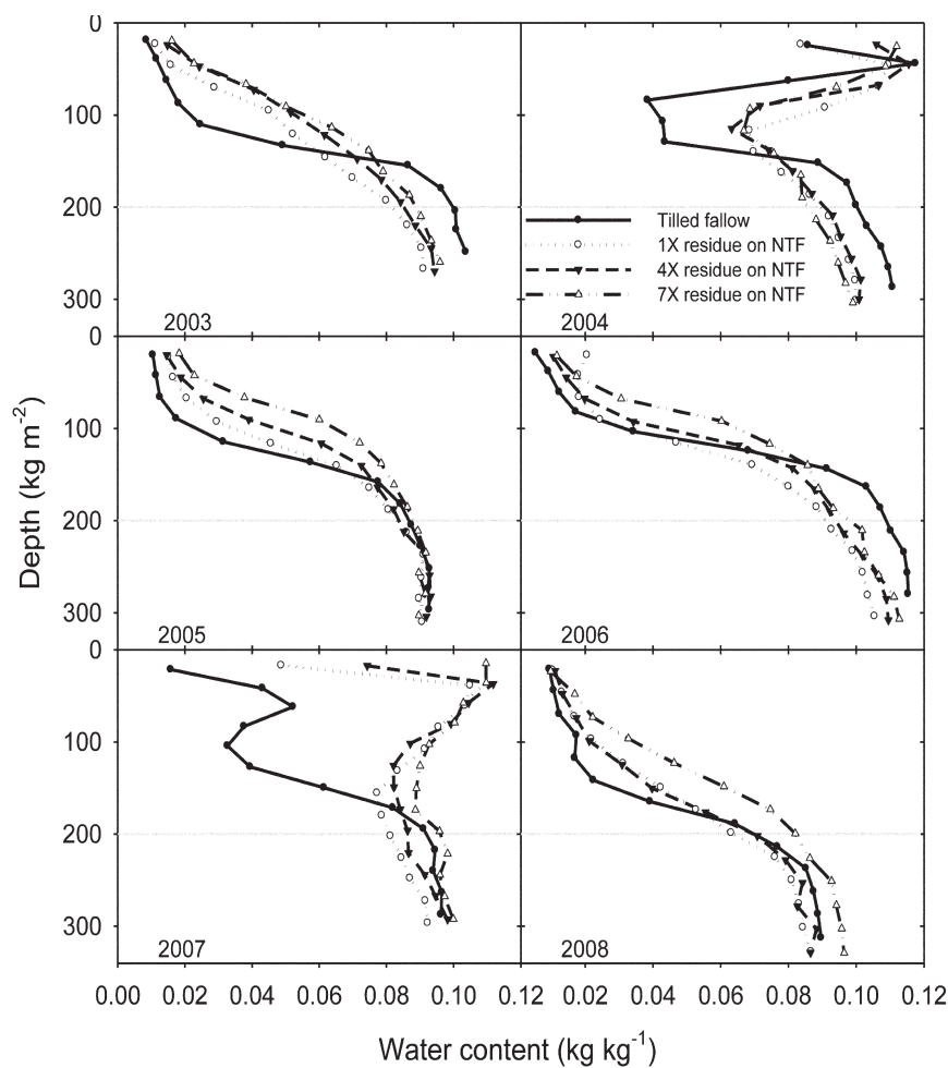
Fig. 2. Seed-zone water content profiles measured in late August from 2003 to 2008. Samples were taken in 2-cm increments from 0- to 26-cm depth (22 cm in 2003) and are plotted on a dry soil mass per area basis. The horizontal guideline marks 200 kg m -2 used for equivalent-mass treatment comparisons. NTF = no-till fallow.
